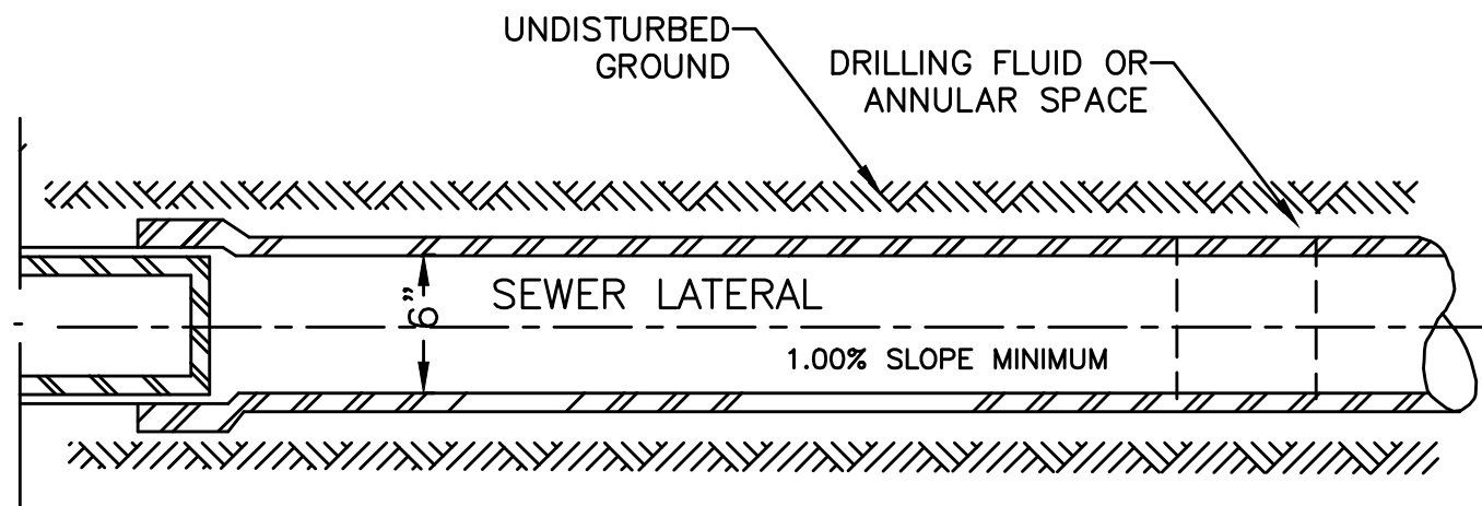
6" LATERAL BORING
