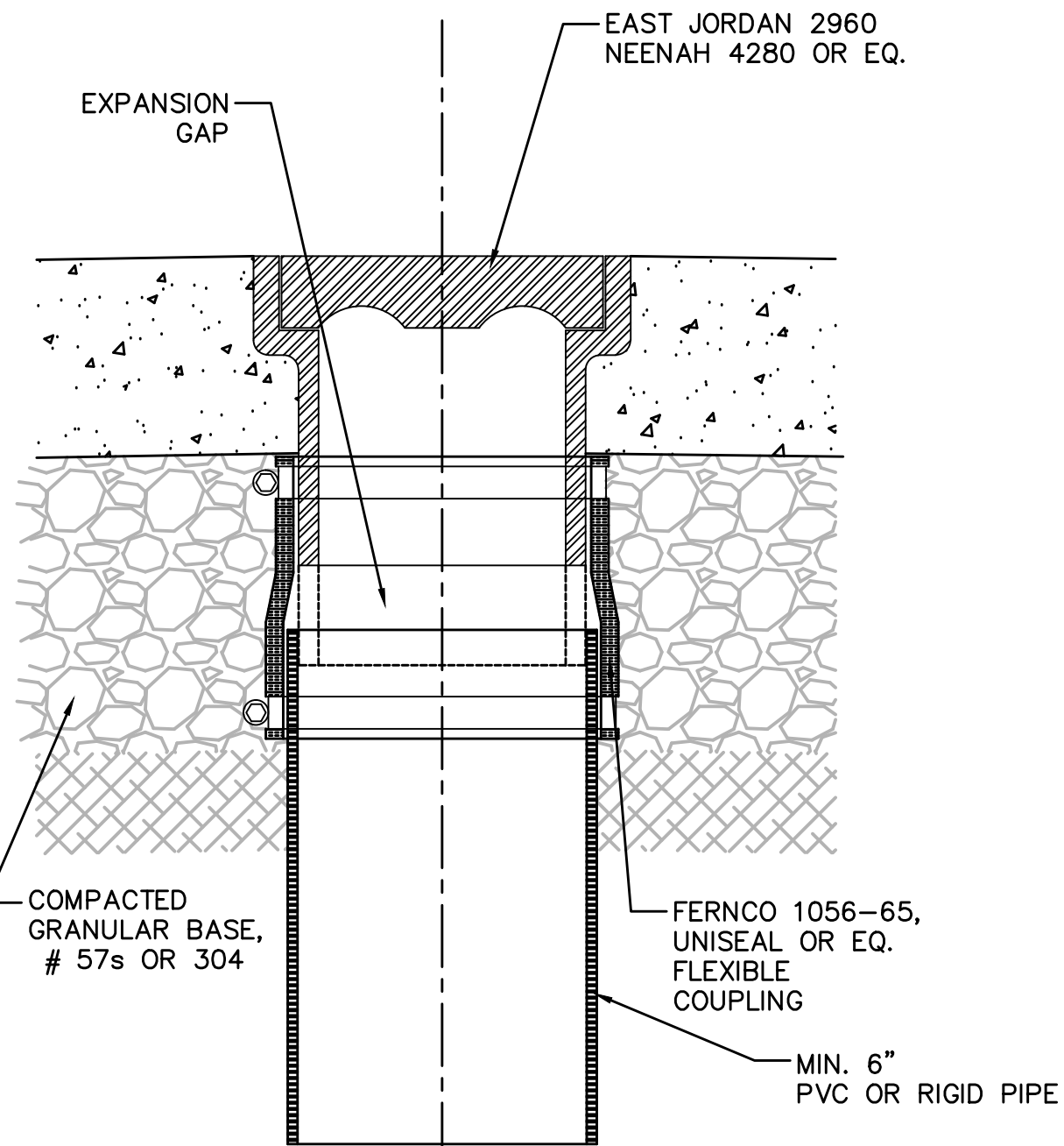
TEST TEE/CLEANOUT COVER IN PAVEMENT
