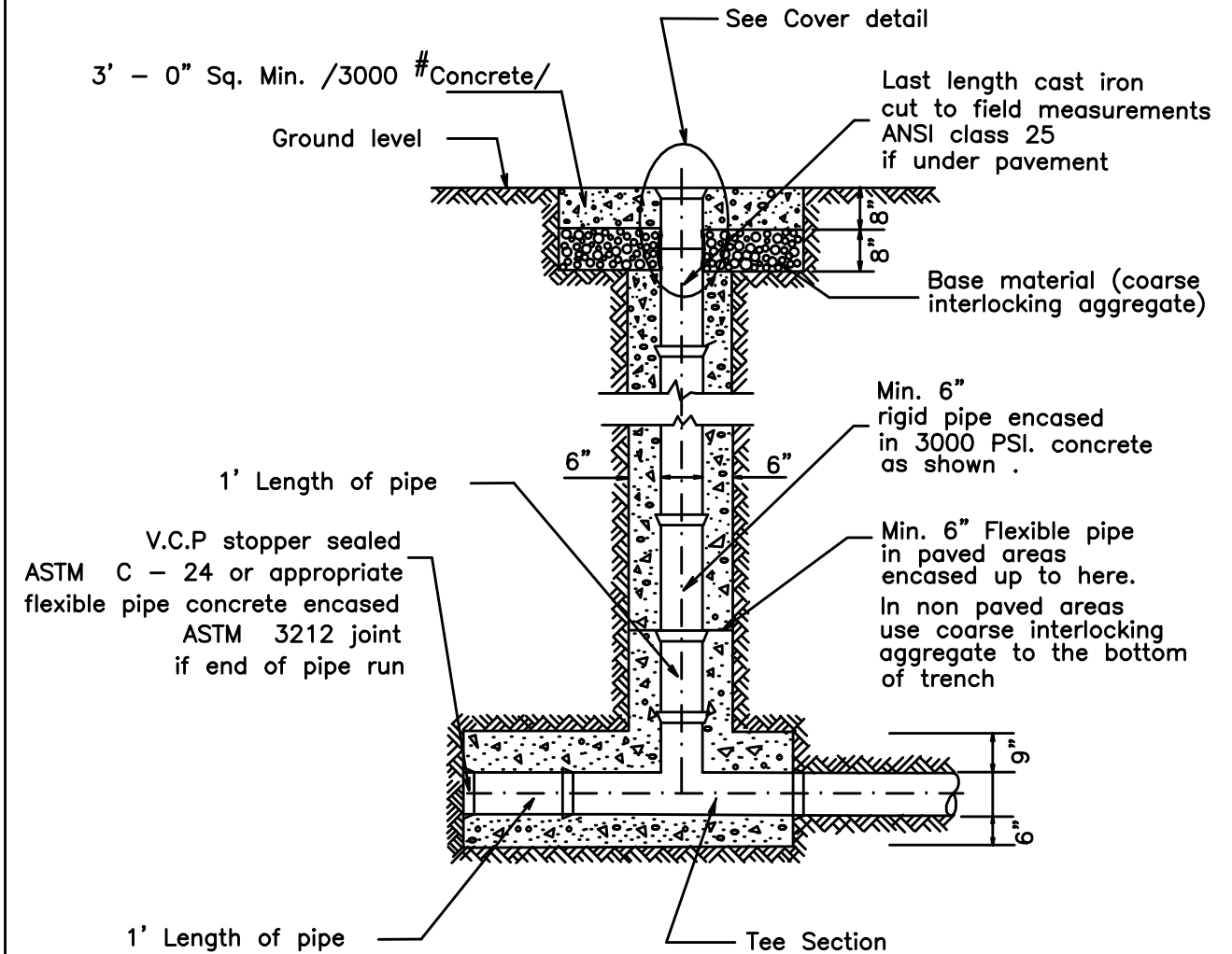
STRAIGHT FLUSH HOLE
