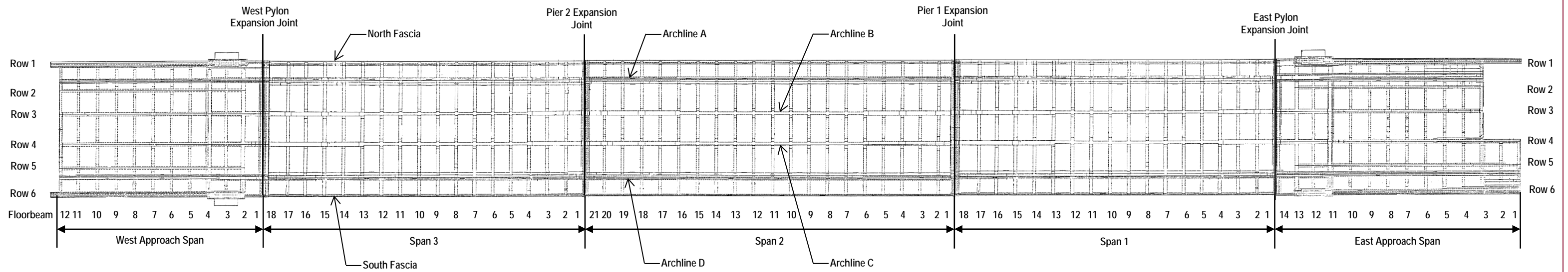
Hilliard Road Bridge Framing Plan
