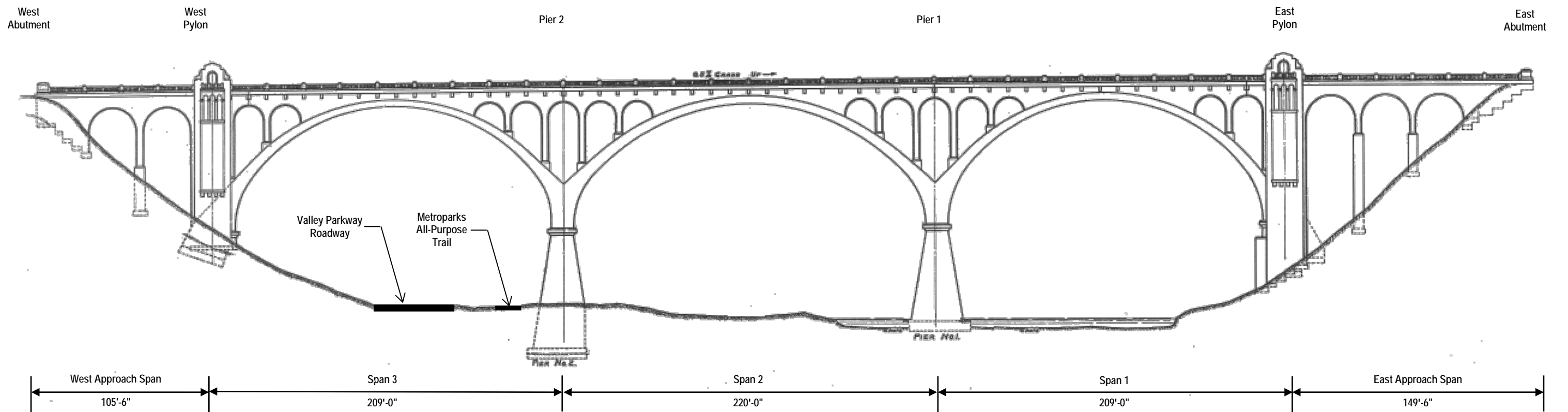
Hilliard Road Bridge South Elevation
