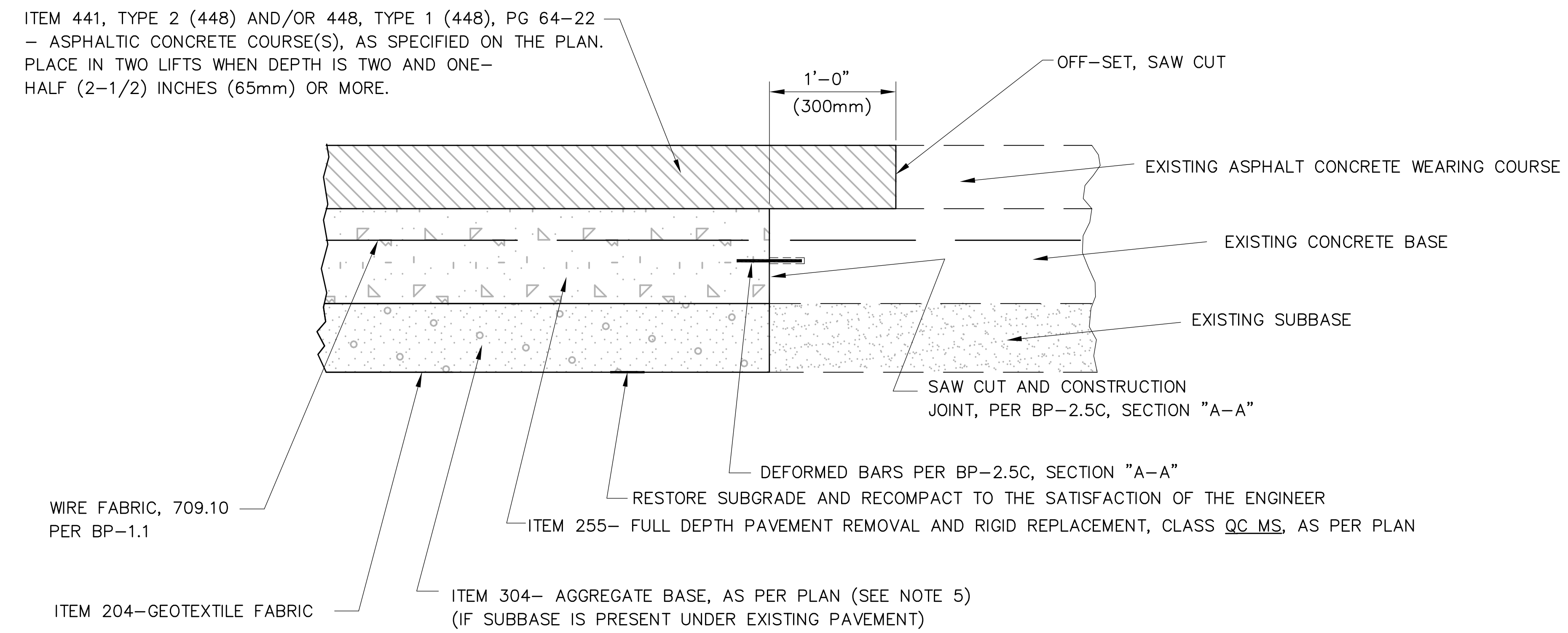
DETAIL-"A" CONCRETE BASE/ASPHALT OVERLAY
